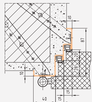
Profil 84_M BRMB = DLB + 80 mm BRMH = DLH + 40 mm
