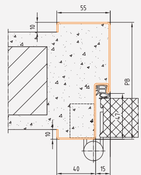
Profil 43_M BRMB = DLB + 130 mm BRMH = DLH + 65 mm
